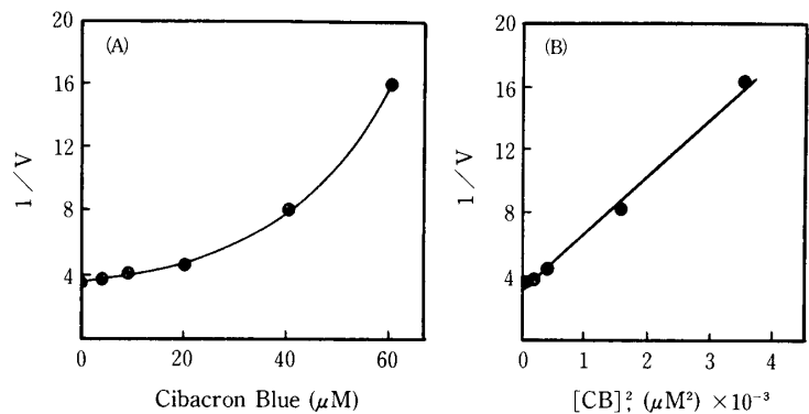
Fig. 8. Effect of Cibacron Blue F3GA on Candida pyruvate kinase. (A) : plots of the reciprocal of the initial velocity with respect to Cibacron Blue F3GA concentration at unsaturated levels of both PEP (0.05 mM) and ADP (0.1 mM). The FDP concentration was 0.5 mM. (B) : replots of the reciprocal of the initial velocity against the square of the Cibacron Blue F3GA concentration. The data from Fig. 8(A) were replotted.
