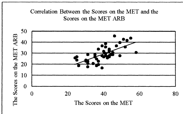
Graph 3: Correlation Between the Scores on the MET and the Scores on the MET ARB in 2005
